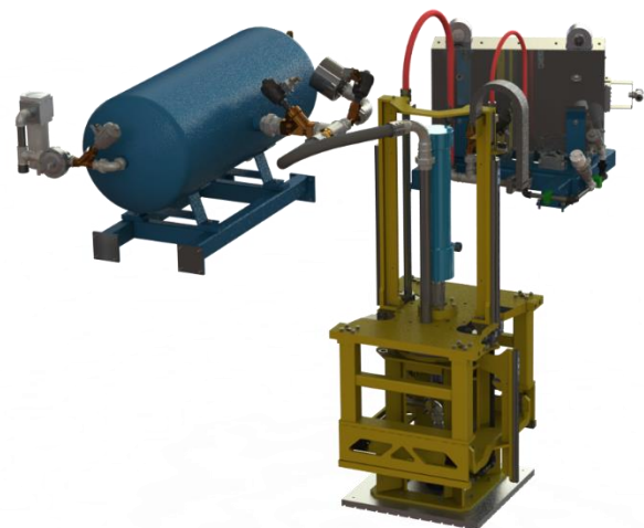
efficient gassing system due to split supply of catalyst and purge air (patented)
